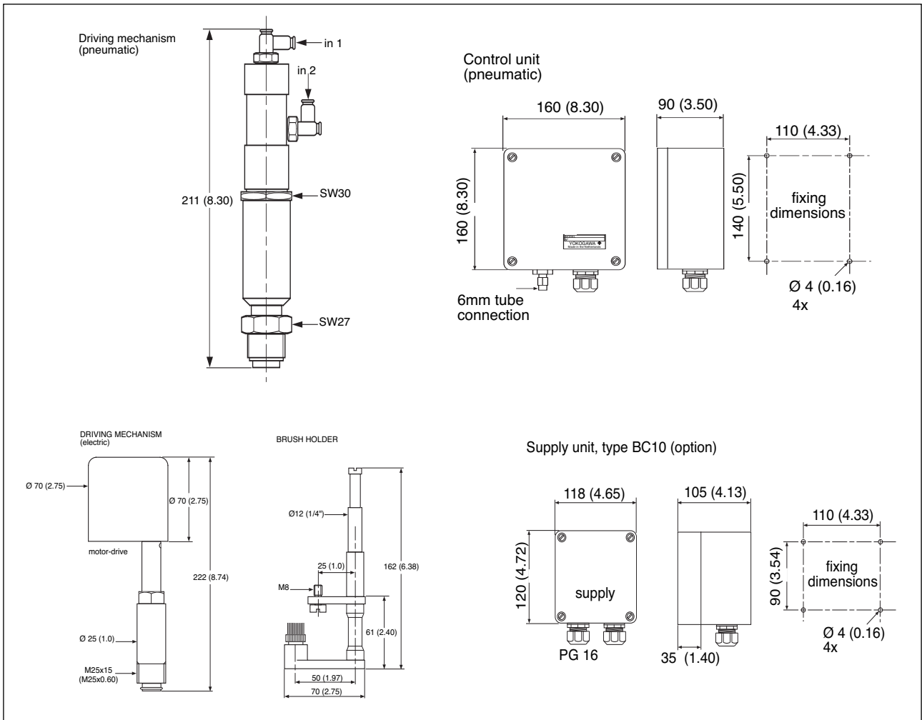
Figure 3. Dimensions
